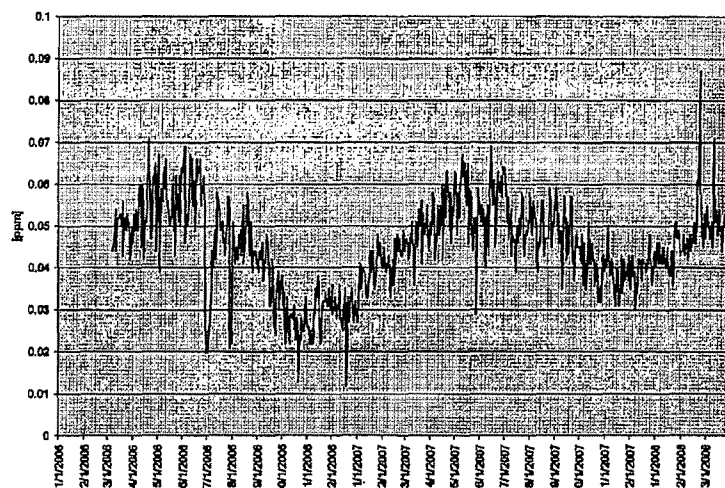
Figure 1. Daily Maximum 8-hr Ozone Values at Wamsutter AQS Site (ID 56-037-0200).
