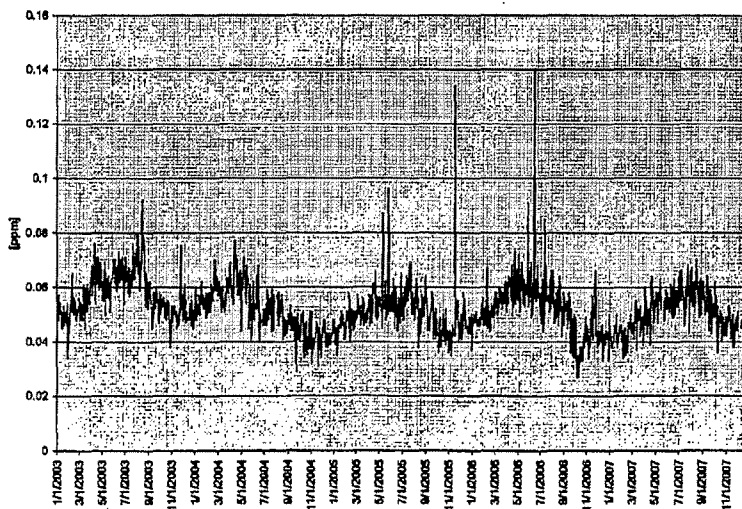
Figure 2. CASTNET Monitor CNT169 (Centennial, WY) 8-hour Daily Maximum Ozone, Years 2003-2007.
