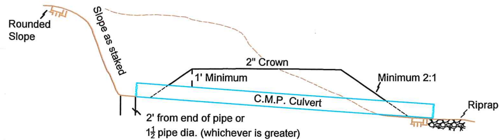
C.M.P. CULVERT INSTALLATION
