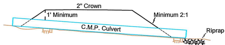
C.M.P. CULVERT INSTALLATION EMBANKMENT SECTION
