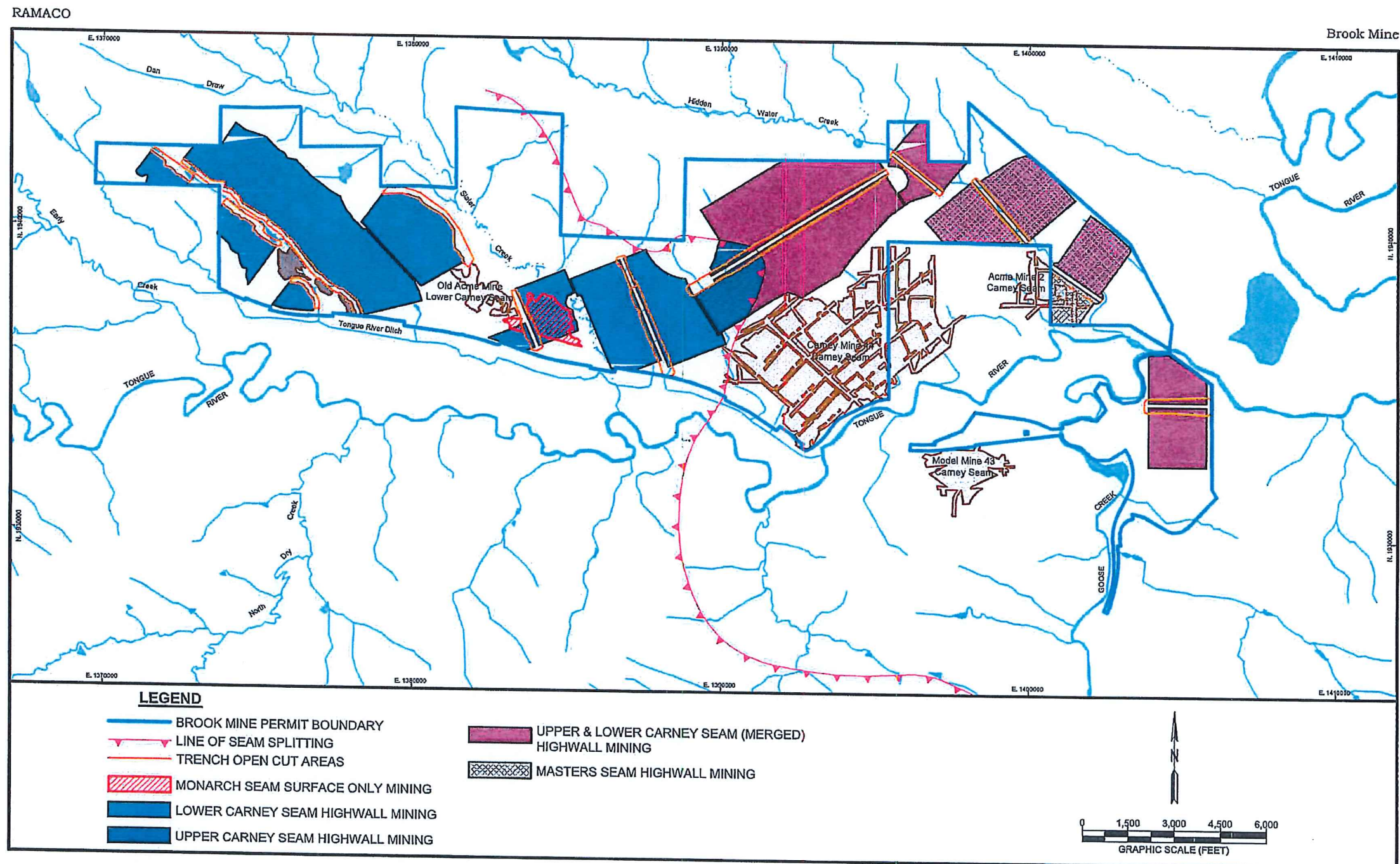
Figure MP-6.1-1 Showing Brook Mine Proposed Trenches and Highwall Mining Panels
