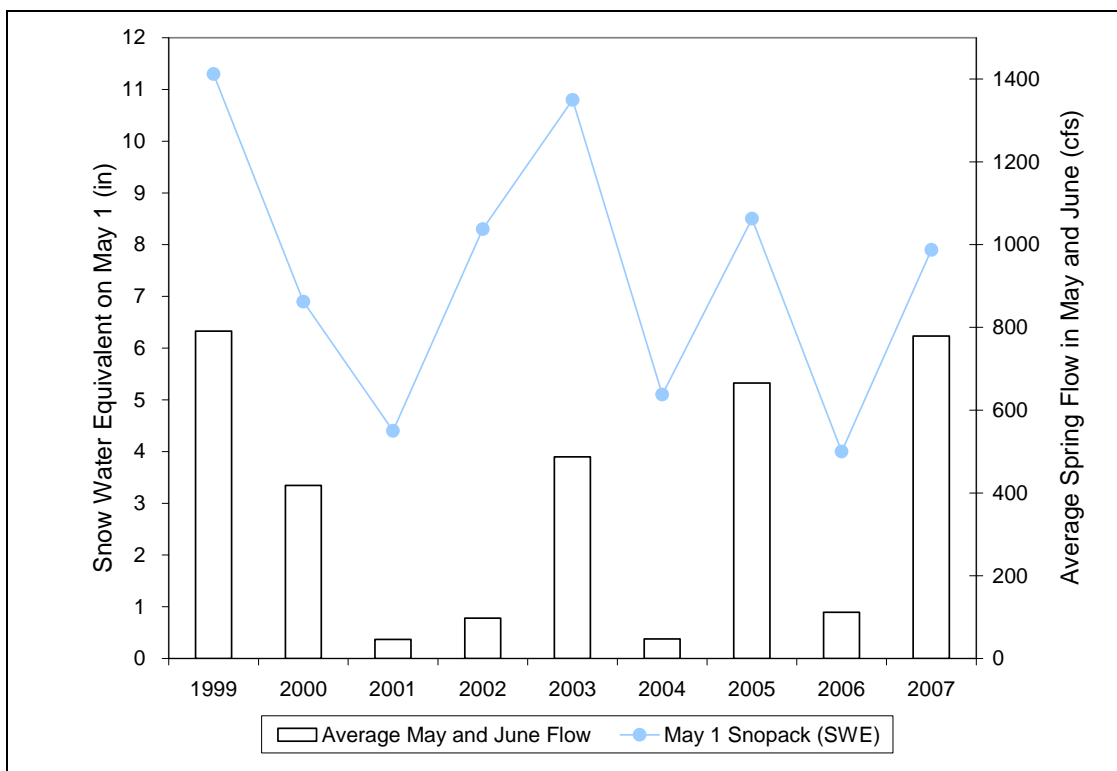
Figure 4.8 Relationship between May 1 snowpack (snow water equivalent) and average spring flow.
