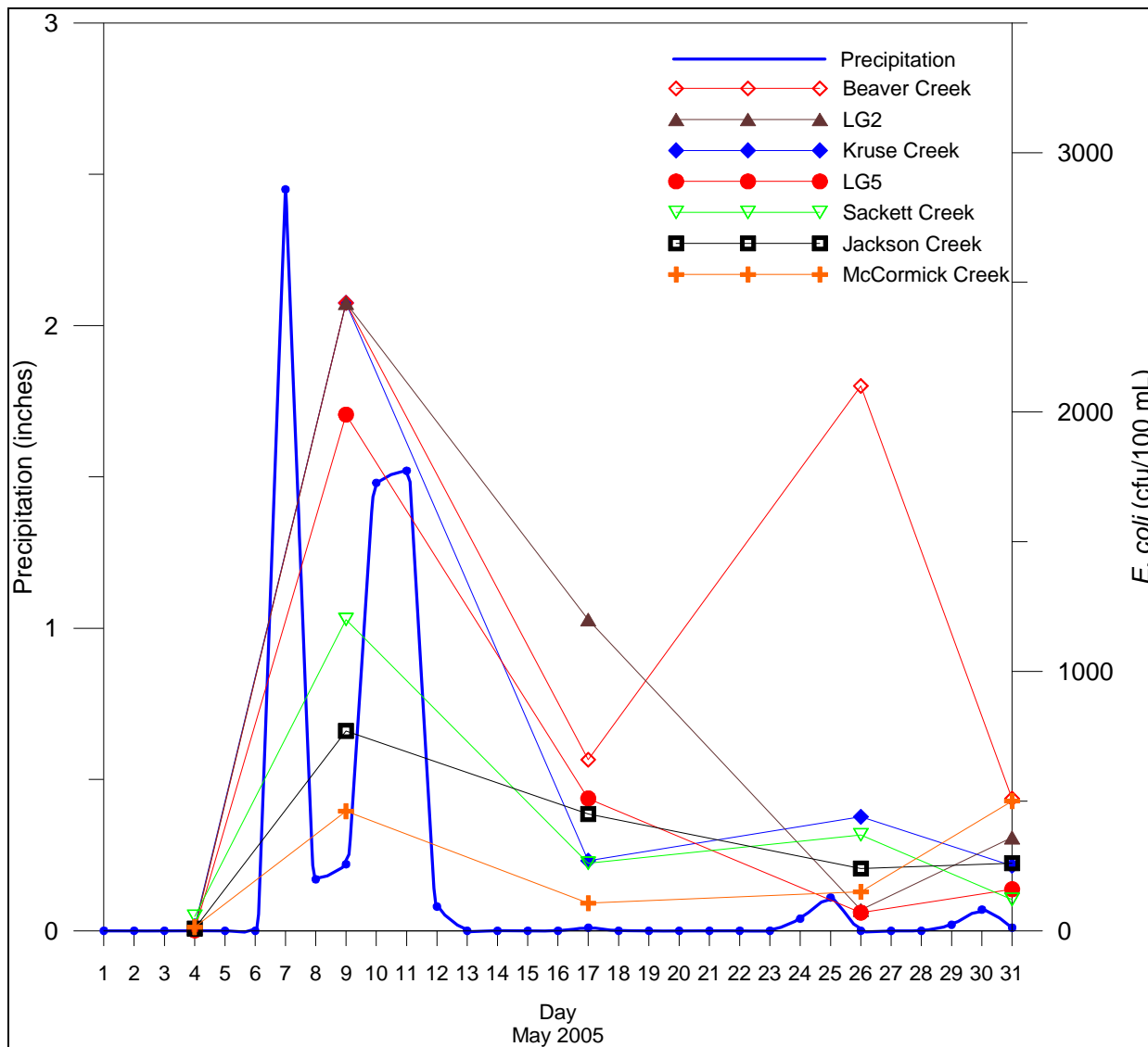
Figure 6.4 May 2005 storm event and E. coli concentrations.
