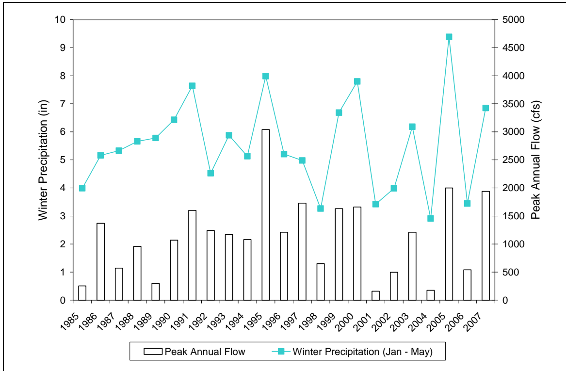
Figure 4.7 Relationship between winter precipitation and peak annual flow.
