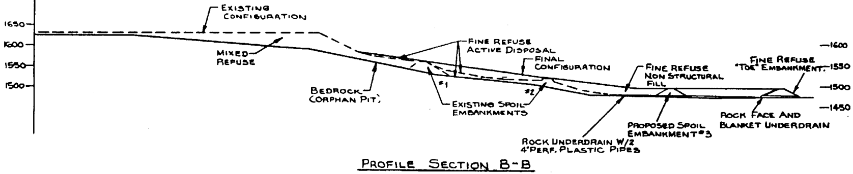
PROFILE CROSS SECTIONS REFUSE AREA #1
